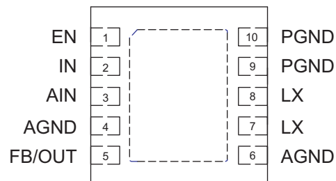
TDFN-10 (Top View)
